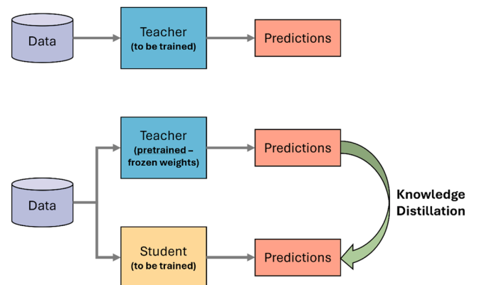
Fig. 6. A schematic framework of offline knowledge distillation.
